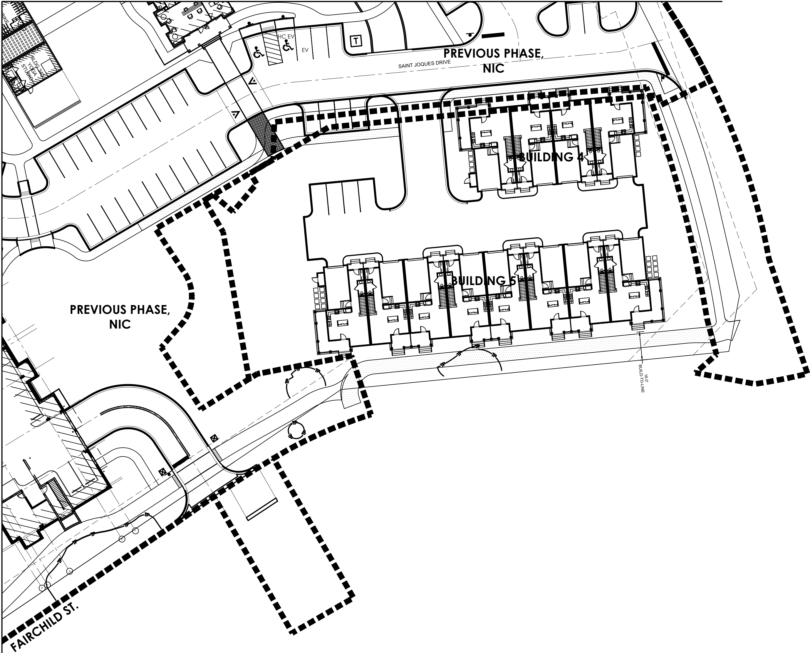
1 ARCHITECTURAL SITE PLAN 1/32" = 1'-0"
